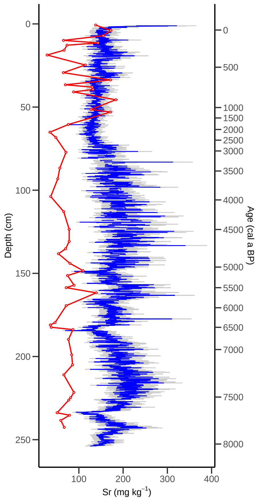
KER1: PLSR Sr Predictions with Confidence Intervals
